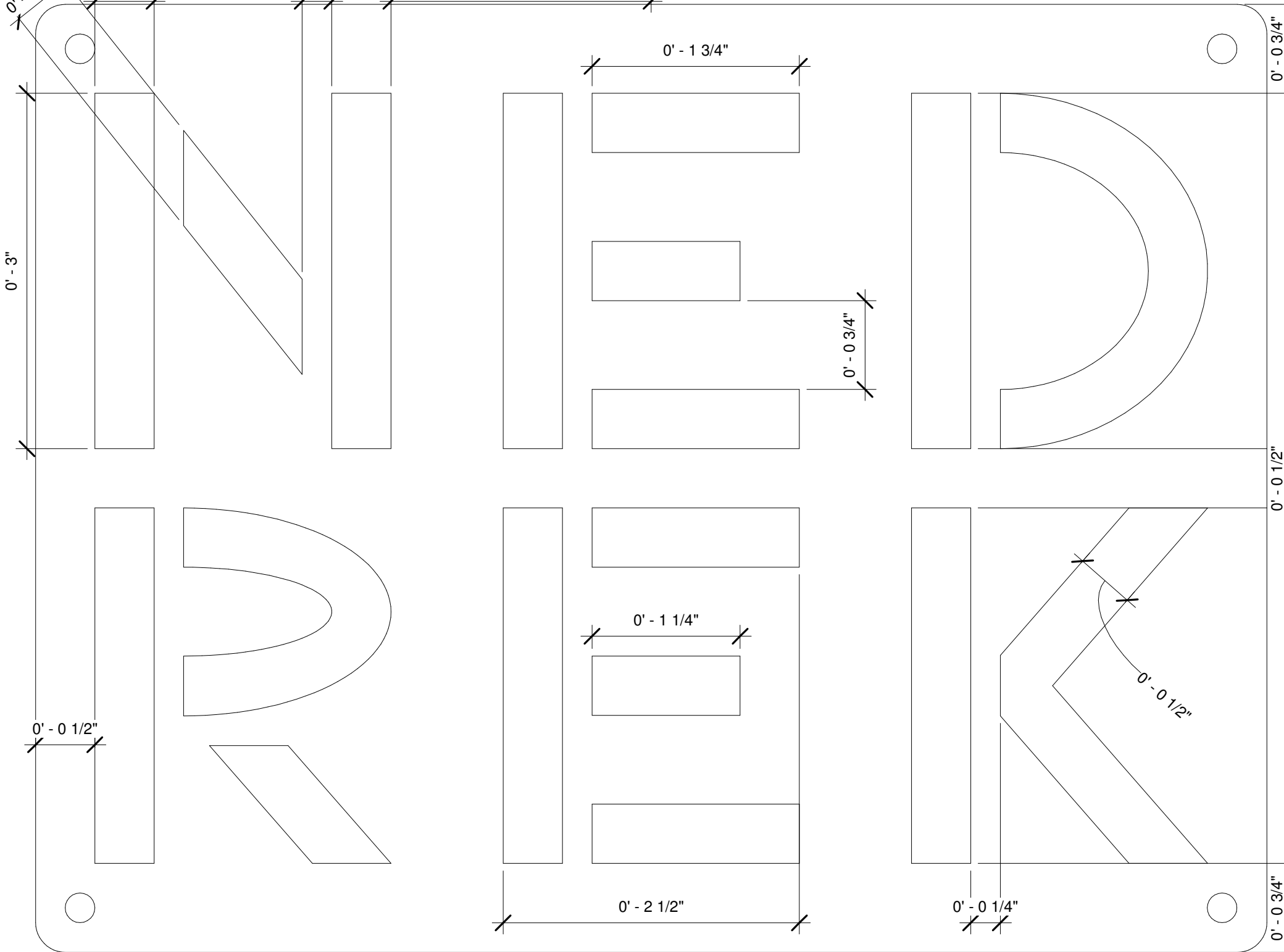
1 1 LEFT (DRIVER) NED REK 12" = 1'-0"
